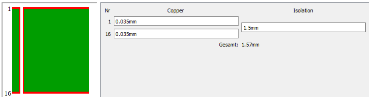
Figure 32: Stack-up
