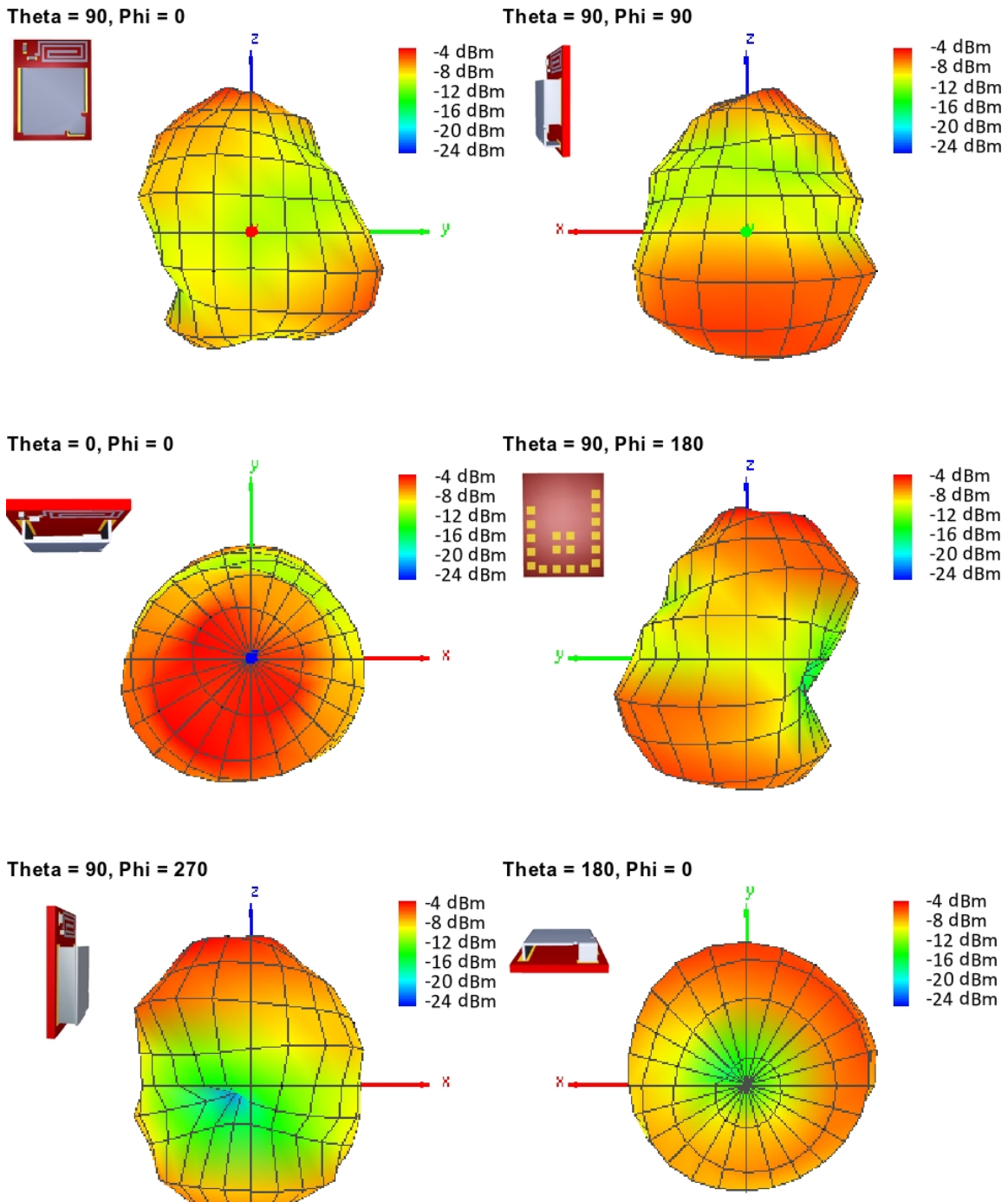
Figure 31: Antenna characteristic from integrated antenna measured on official EV-Board 1
