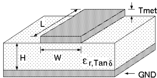
Figure 27: Dimensioning the antenna connection as micro strip
